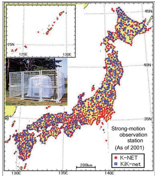
Figure 1 : Location of Strong-Motion Observation Stations K-NET and KiK-net. (Reprint from Ref. 1)
