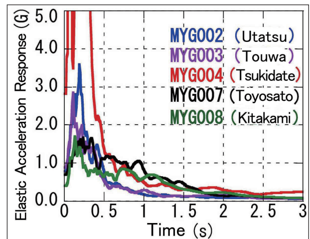
Figure 5 : Spectrum of the Elastic Acceleration Response at Other Observation Stations. (Provided by Y. Sakai)
