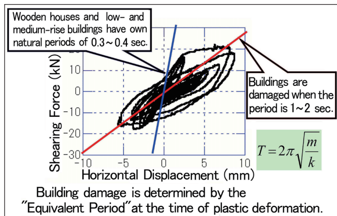
Figure 6 : Result of Model Experiment (Provided by Y. Sakai)
