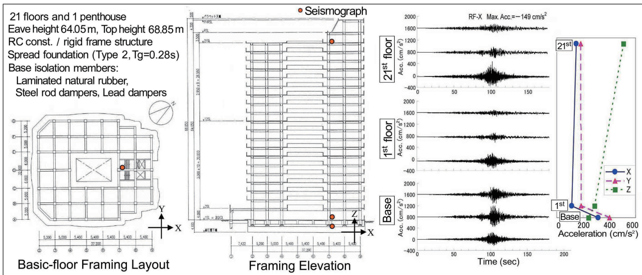
Figure 16 : Observed Motion of a Super-high Rise Building with Seismic Isolation during the 2011 Tohoku Earthquake. (Provided by S. Sakai)
