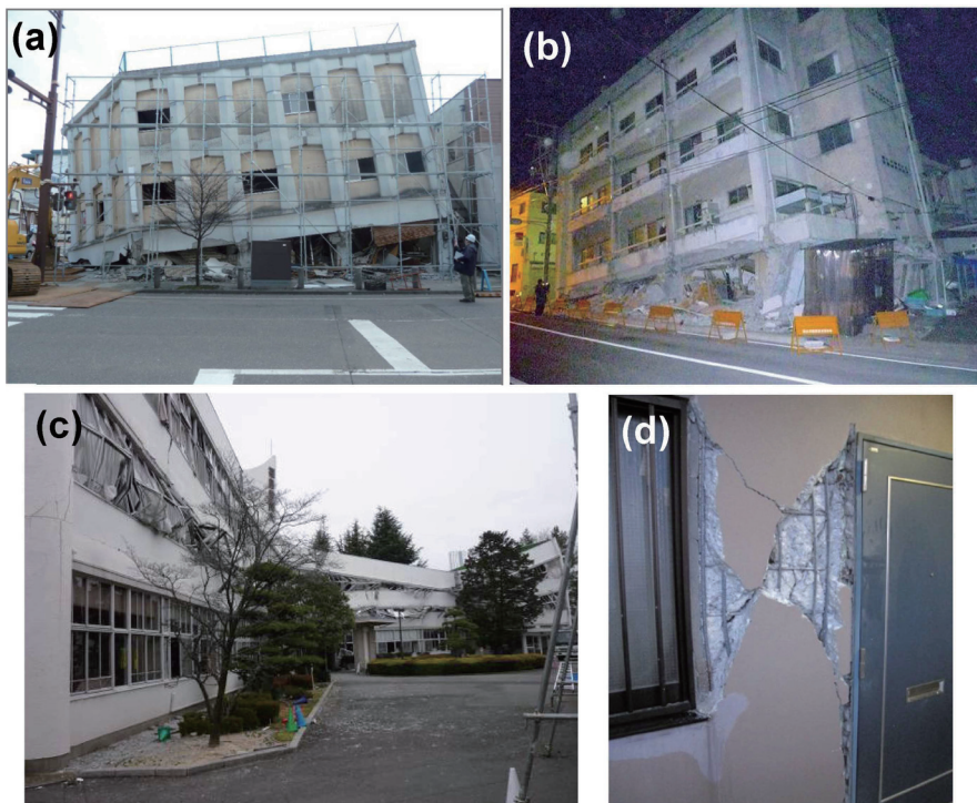
Figure 9 : Examples of building damage due to the 2011 Tohoku Earthquake. (Reprint from Refs. 3 and 4)
