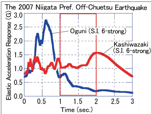
Figure 10 : Spectrum of Elastic Acceleration Response in the 2007 Niigata Pref. Off-Chuetsu Earthquake. (Provided by Y. Sakai)
