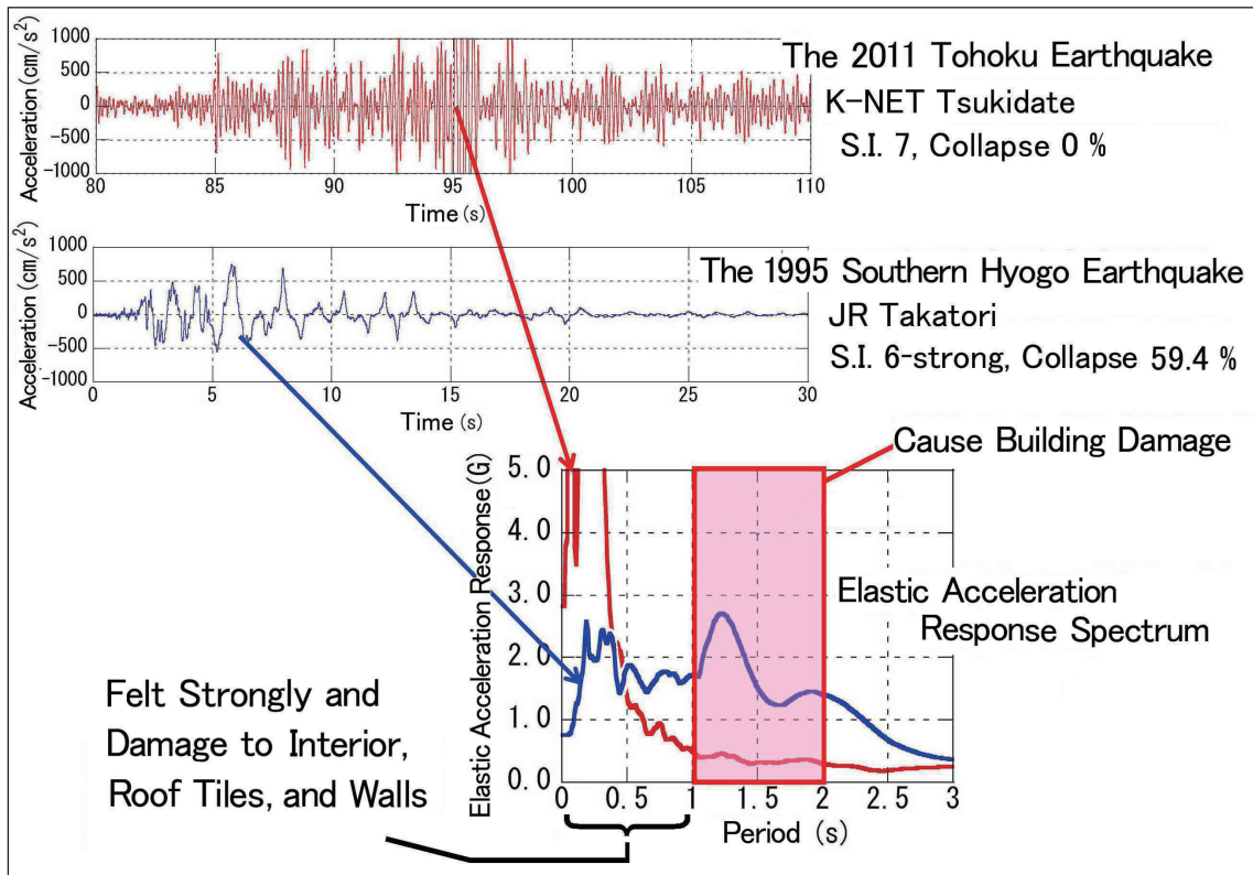
Figure 4 : Comparison of Ground Motions in the 2011 Tohoku Earthquake and the 1995 Southern Hyogo Prefecture Earthquake. (Provided by Y. Sakai)
