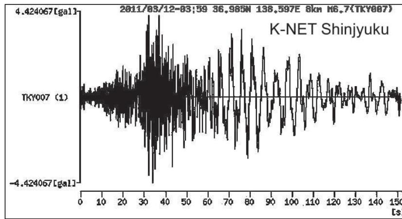
Figure 17 : Aftershock Ground Motion Observed at Shinjuku (from Ref.2)
