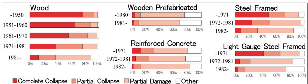
Figure 7 : Damage Situation of Buildings in Ashiya City (Reprint from Ref. 6)
