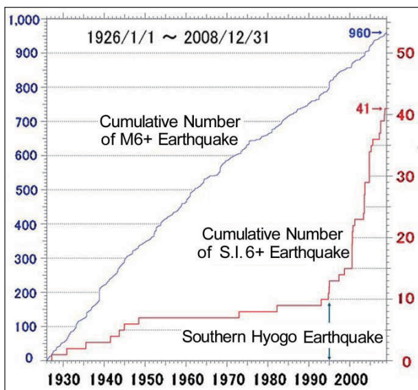
Figure 12 : Cumulative Number of Large Earthquakes. (Reprint from Ref. 10)
