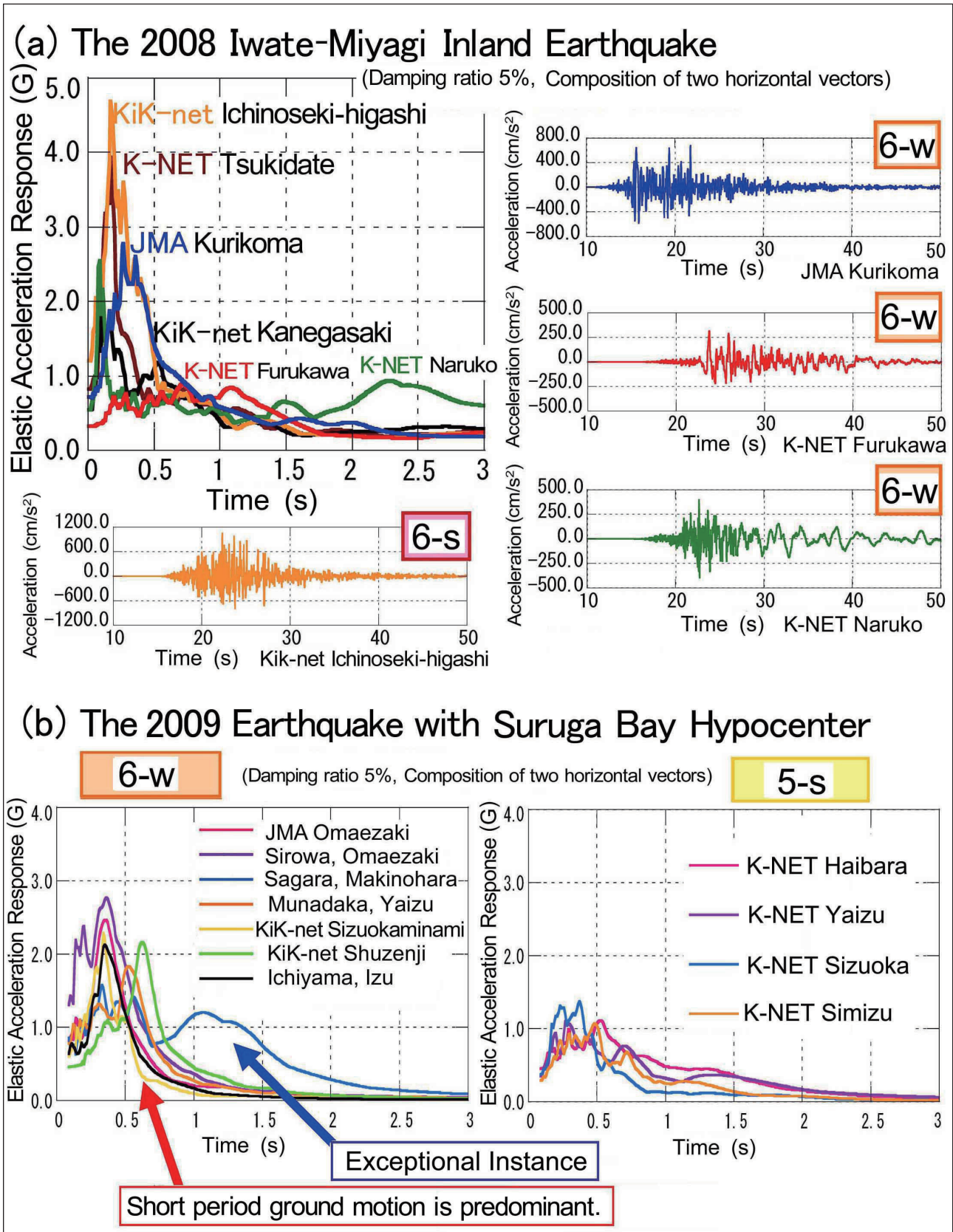
Figure 11 : The Elastic Acceleration Response Spectra in Two Major Earthquakes. (Provided by Y. Sakai)
