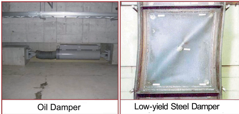
Figure 14 : Types of Inter-Floor Dampers. (Provided by S. Sakai)
