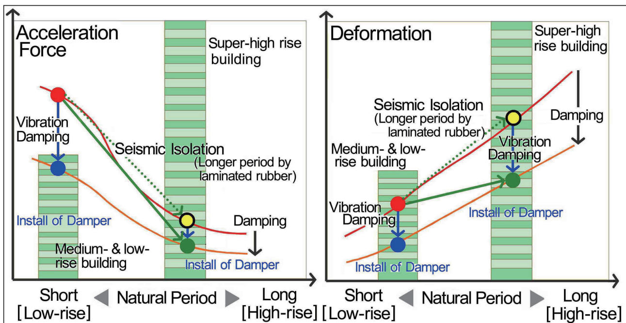
Figure 13 : Force Applied to Buildings and Deformation of Buildings. (Provided by S. Sakai)
